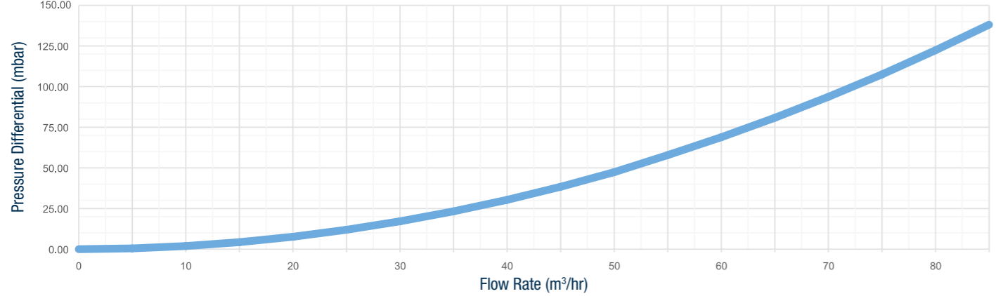
4" BoilermagXT BMXT200/4/AAV
