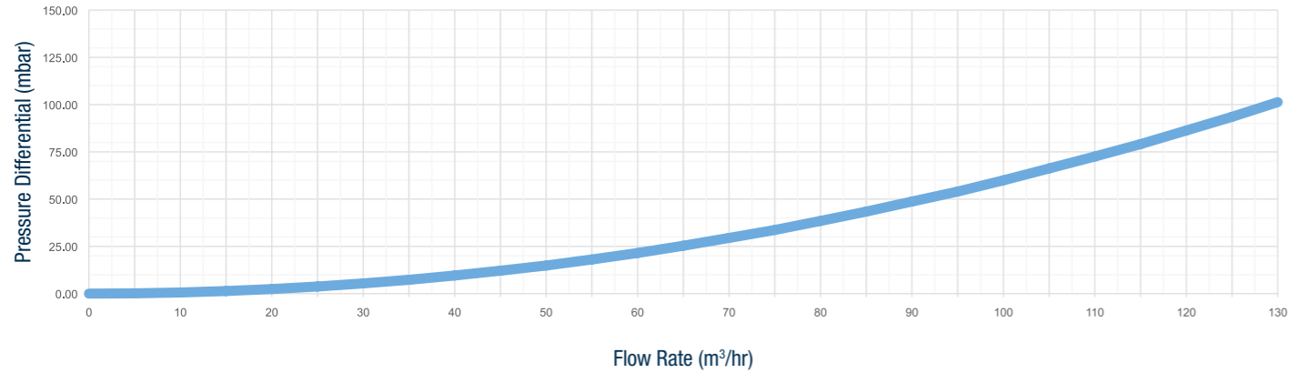
4" BoilermagXT BMXT200/4/AAV
